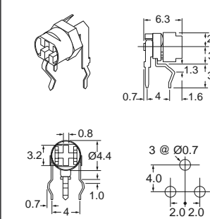
Fig. 4 — 6mm, Vertical
