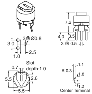
Fig. 3 — 5mm, Vertical
