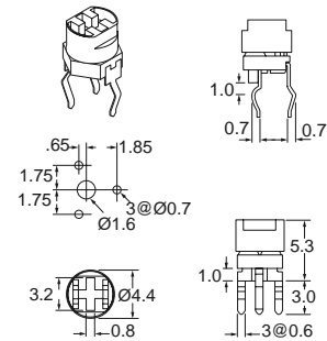
Fig. 3 — 5mm, Vertical
