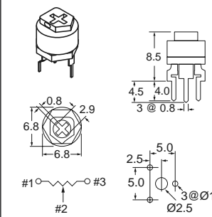
Fig. 4 — 6mm, Vertical
