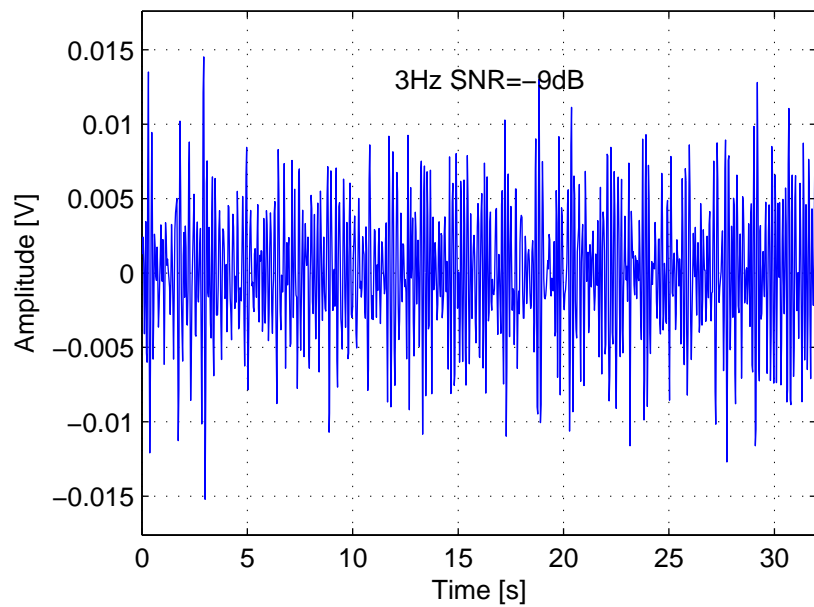
Noise corrupted Filter Output
