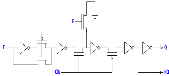
Schematic for Dynamic T Flip Flop with Reset and Enable
