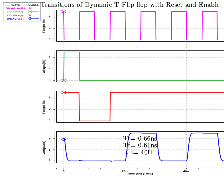
Hspice file created from tff6_50
